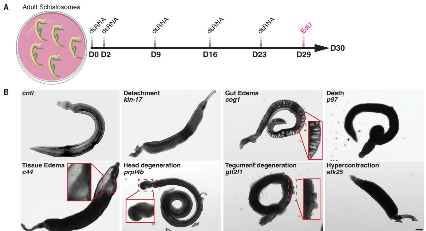
Fig. 1. Summary of RNAi phenotypes. (A) RNAi treatment regimen. Parasites were monitored for visible abnormalities, and at day 29 EdU was added to medium to label proliferative cells. (B) Categories of RNAi phenotypes observed. kin-17 (Smp_023250), cog1 (Smp_132980), p97 (Smp_018240), c44 (Smp_136260), prpf4b (Smp_068960), gtf2f1 (Smp_088460), stk25 (Smp_096640). Scale bar, 100 \mu m.
